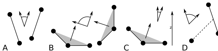
Fig. 5.56: Angle options of gmx gangle (page 188): A. Angle between two vectors. B. Angle between two planes. C. Angle between a vector and the z axis. D. Angle between a vector and the normal of a sphere. Also other combinations are supported: planes and vectors can be used interchangeably.
